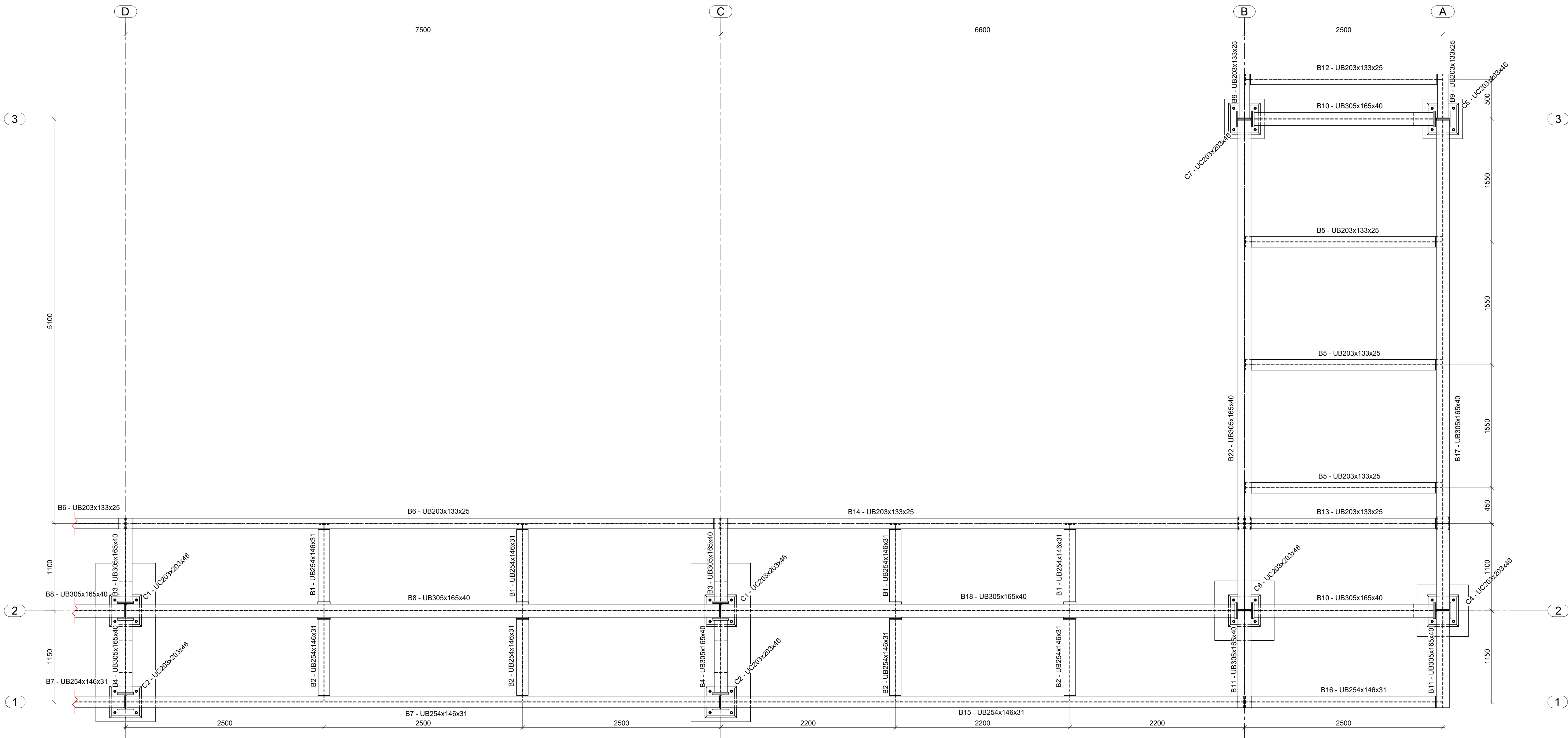
PLATFORM PLAN ON FRAME 2 & 3 GRIDS F TO D FOR ELEVATIONS SEE DRAWING B01388-BH-GF-102 5 of 6
