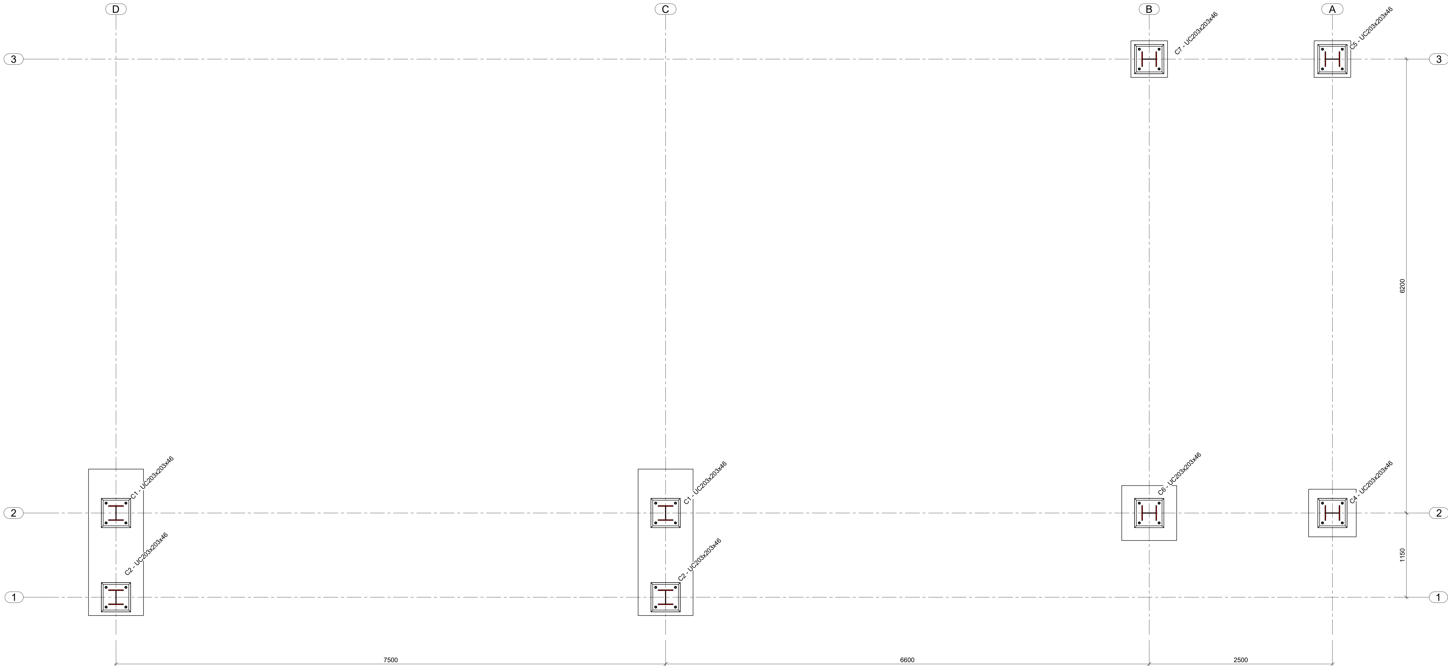
BASE PLATE PLAN ON FRAME 2 & 3 GRIDS D TO A
