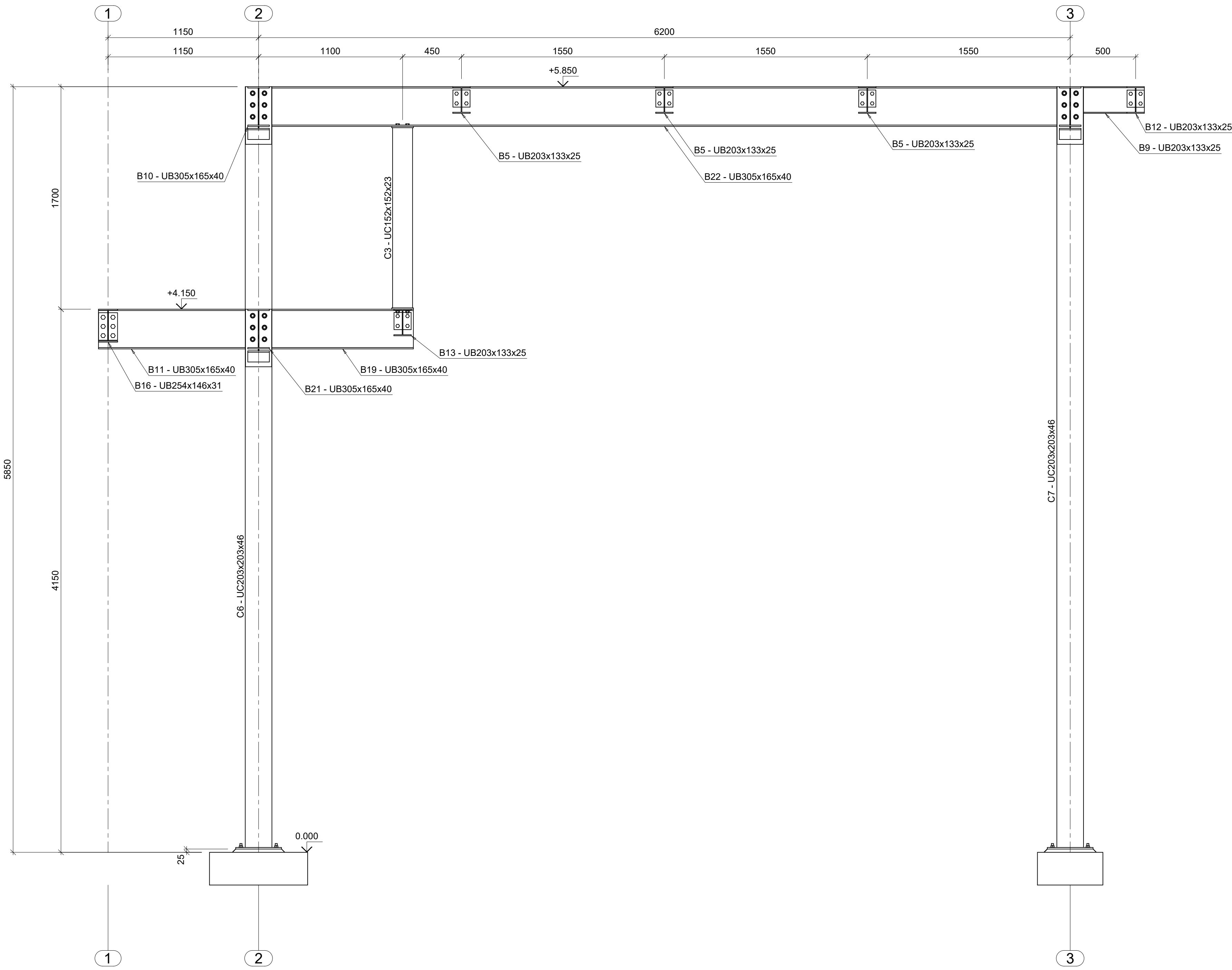
ELEVATION ON FRAME 2 & 3 GRIDLINE B 1 TO 3
