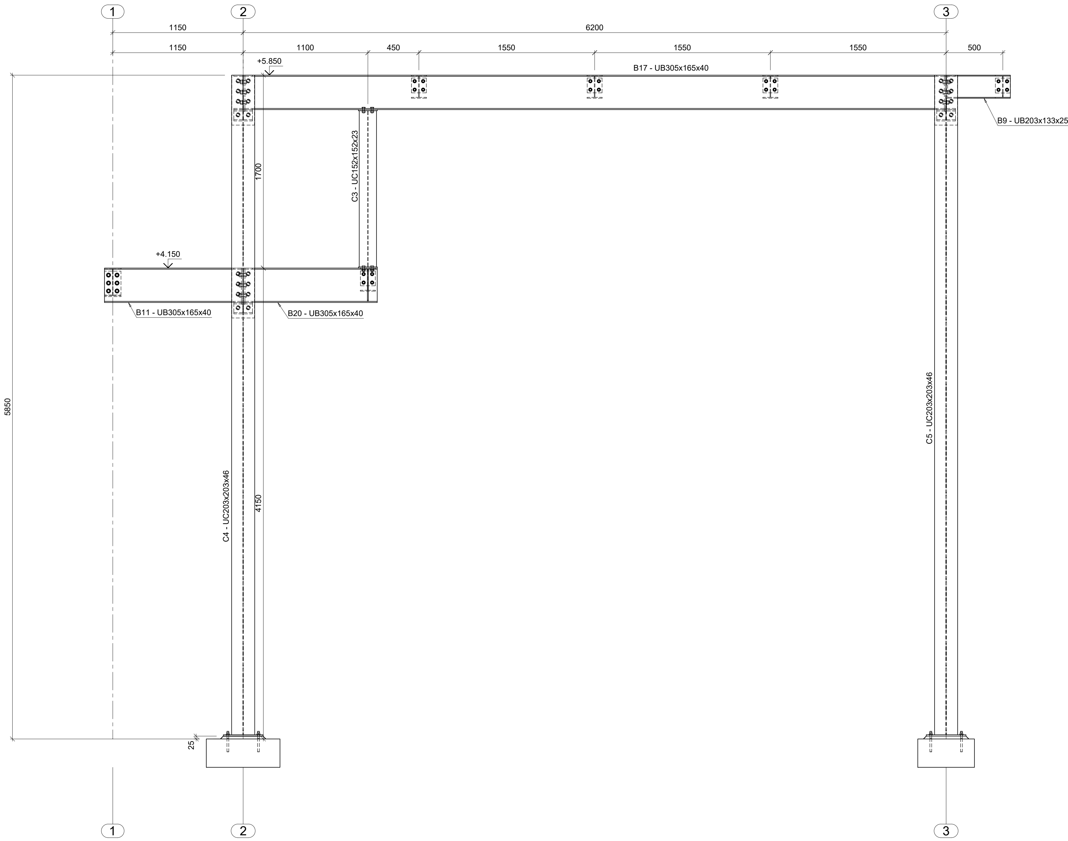
ELEVATION ON FRAME 2 & 3 GRIDLINE A 1 TO 3
